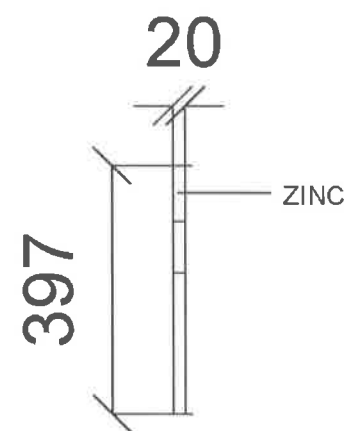
SIDE VIEW unit of mm.
